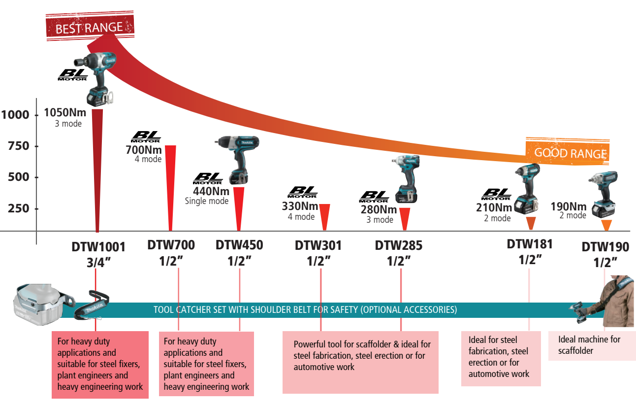
18V LXT - Lithium-Ion Cordless Impact Wrench Comparison Chart
