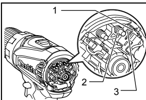
1. Recessed part 2. Spring 3. Arm
